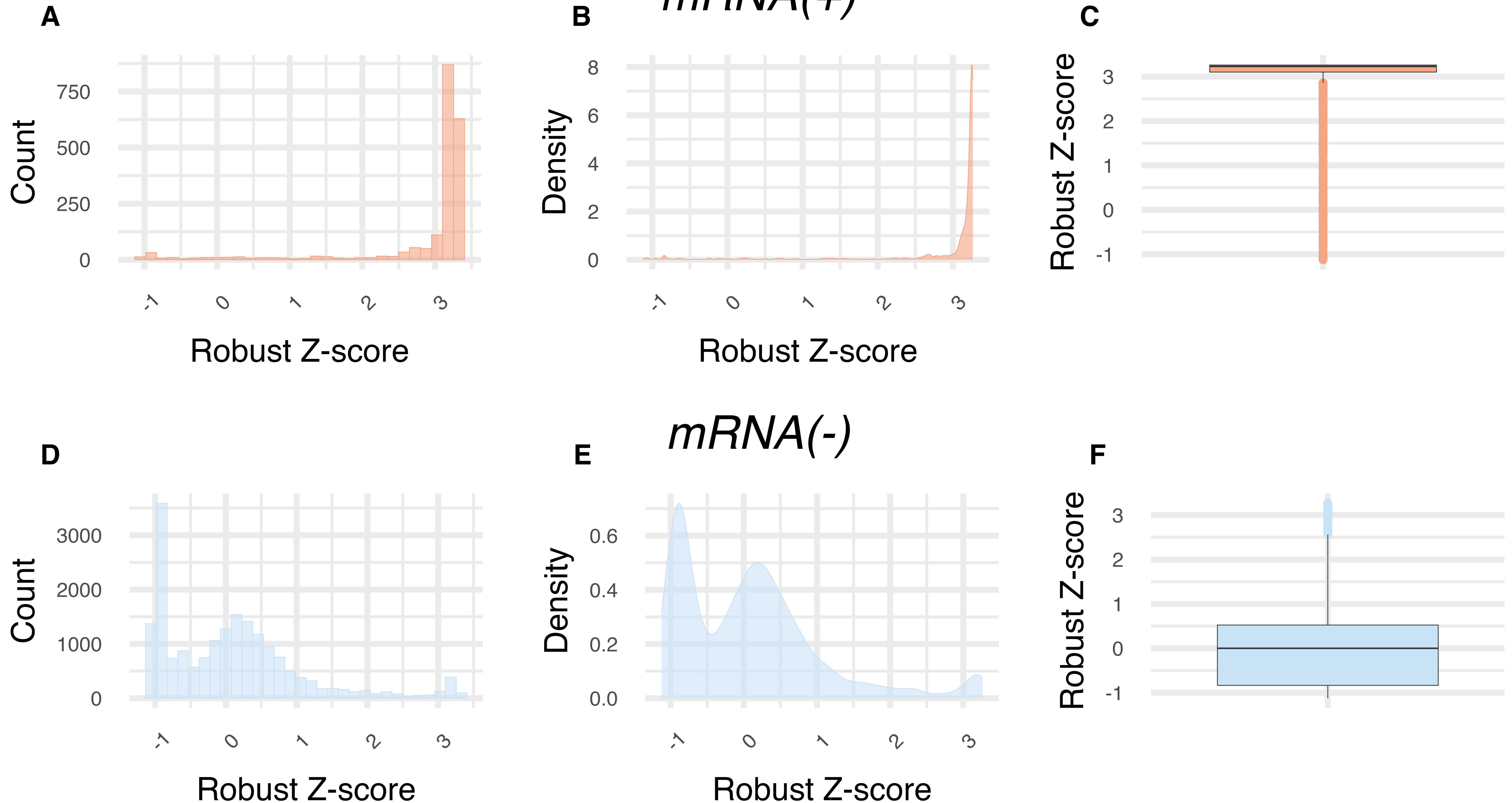
Supplementary Figure S6. mRNA PhyloP mammals robust z-scores distributions. A-C) Histogram, Density and Boxplot for mRNA(+), D-F) Histogram, Density and Boxplot for mRNA(-). The positive dataset show robust z-scores centered around 3, whereas robust z-scores for the negative set are centered around 0, this indicates the two dataset come from different distributions
